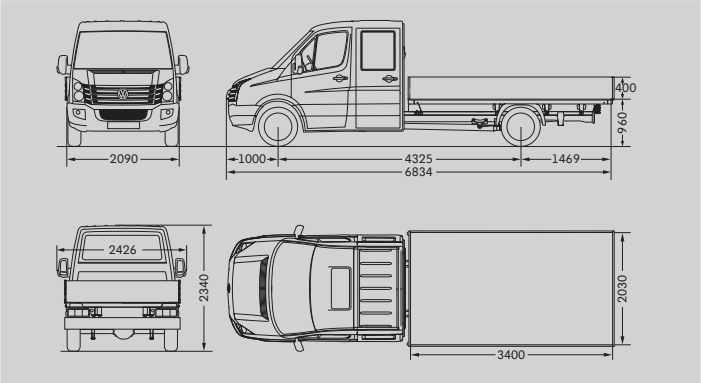
Crafter 35 Dropside Van with double cab and long wheelbase
