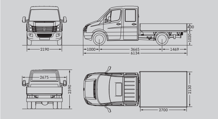
Crafter 50 Dropside Van with double cab and medium wheelbase
