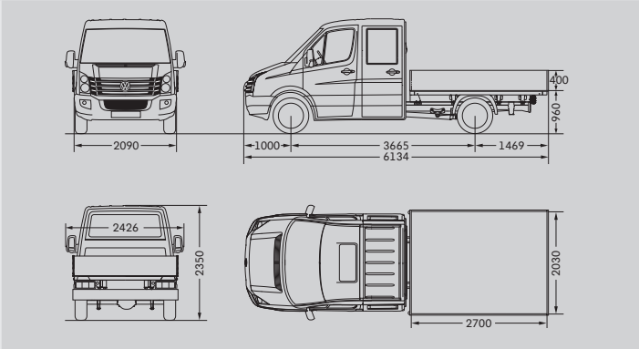
Crafter 35 Dropside Van with double cab and medium wheelbase
