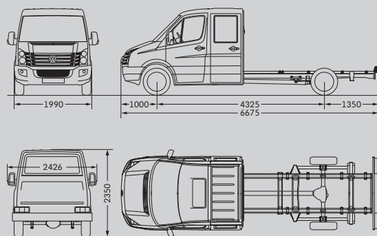
Crafter 35 Chassis with double cab and long wheelbase
