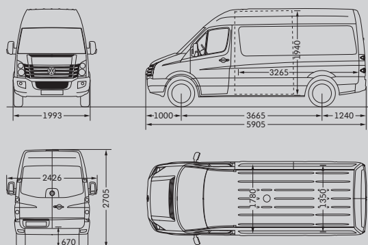
Crafter 30/35 Delivery Van with medium wheelbase and high roof
