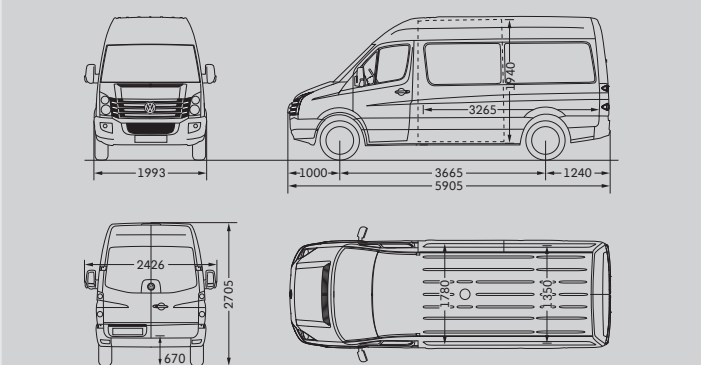
Crafter 30/35 Kombi with medium wheelbase and high roof
