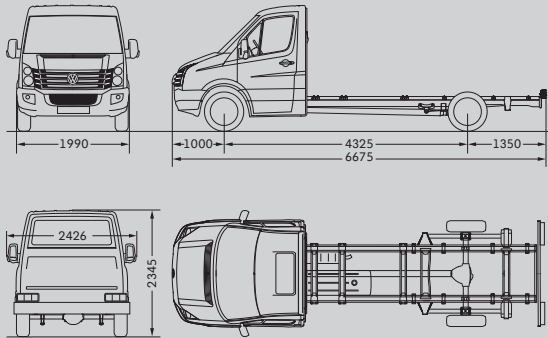
Crafter 35 Chassis with single cab and long wheelbase
