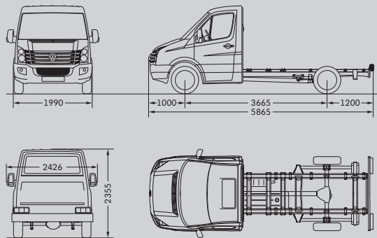
Crafter 30 Chassis with single cab and medium wheelbase
