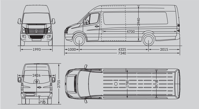
Crafter 50 Delivery Van with long wheelbase, overhang and high roof
