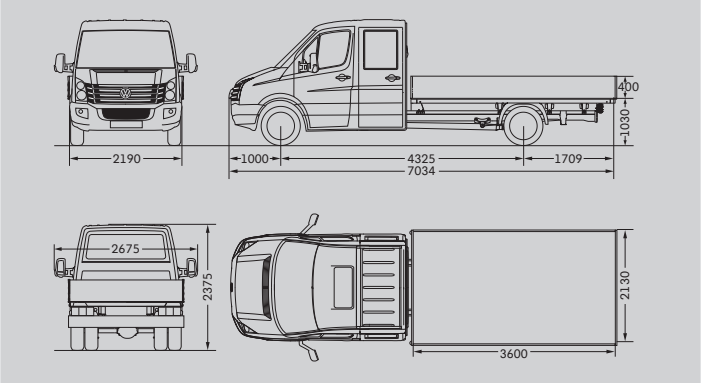
Crafter 50 Dropside Van with double cab and long wheelbase
