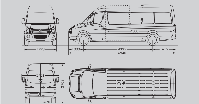
Crafter 35 Kombi with long wheelbase and high roof
