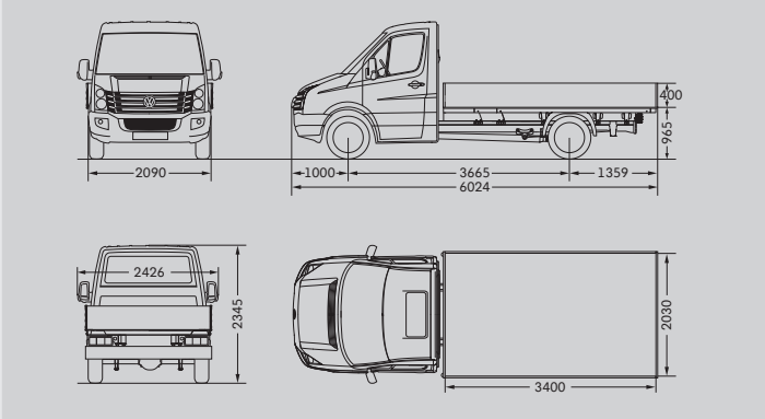
Crafter 30 Dropside Van with single cab and medium wheelbase
