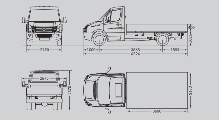
Crafter 50 Dropside Van with single cab and medium wheelbase
