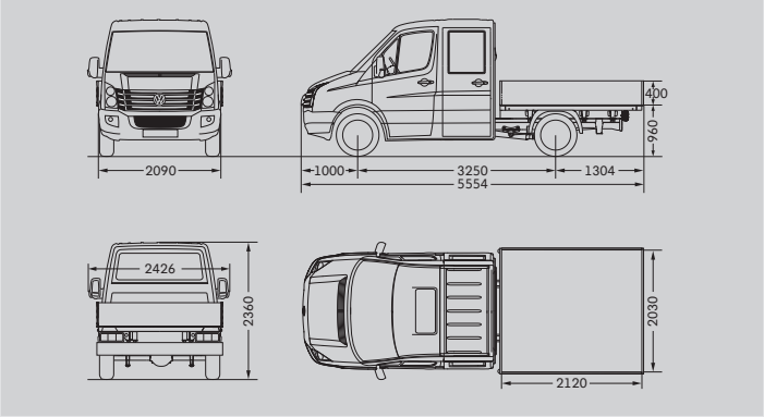
Crafter 35 Dropside Van with double cab and short wheelbase
