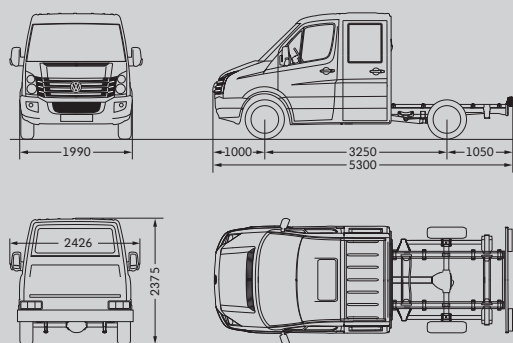
Crafter 30 Chassis with double cab and short wheelbase
