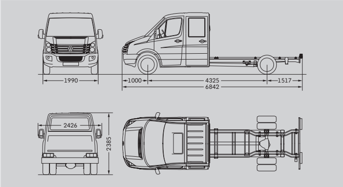
Crafter 50 Chassis with double cab and long wheelbase
