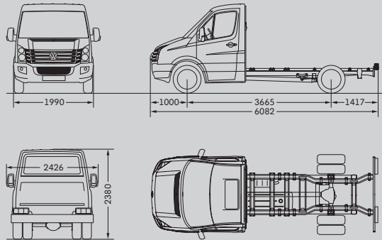
Crafter 50 Chassis with single cab and medium wheelbase
