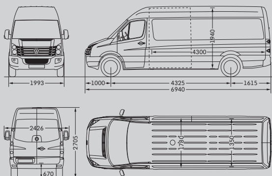
Crafter 35 Delivery Van with long wheelbase and high roof
