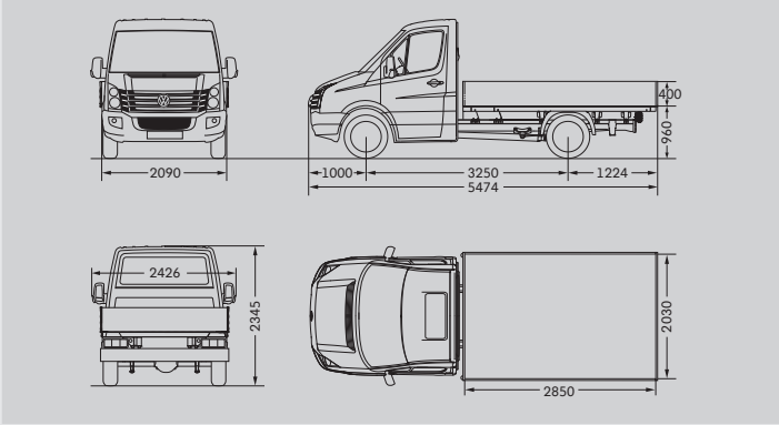
Crafter 35 Dropside Van with single cab and short wheelbase
