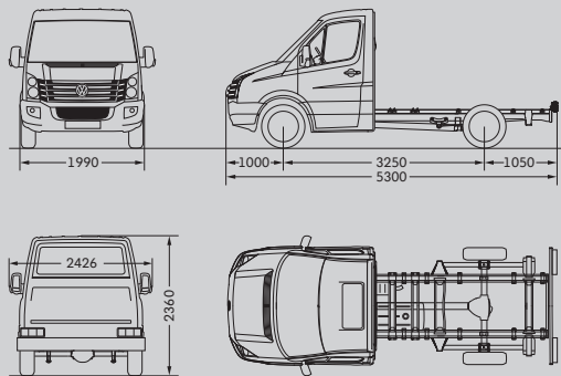
Crafter 30 Chassis with single cab and short wheelbase
