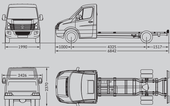
Crafter 50 Chassis with single cab and long wheelbase
