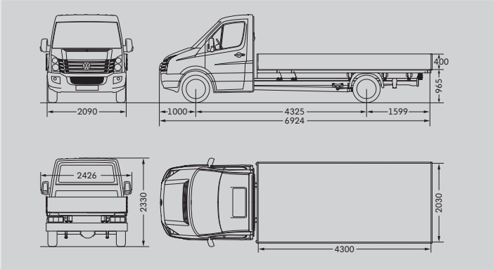
Crafter 35 Dropside Van with single cab and long wheelbase
