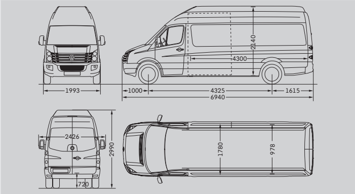
Crafter 50 Delivery Van with long wheelbase and super-high roof
