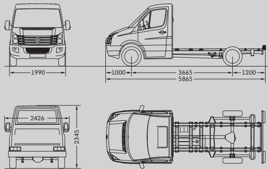
Crafter 35 Chassis with single cab and medium wheelbase
