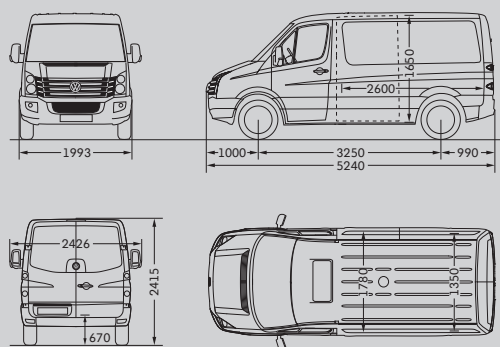
Crafter 30/35 Delivery Van with short wheelbase and normal roof
