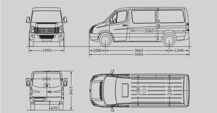
Crafter 30/35 Kombi with medium wheelbase and normal roof
