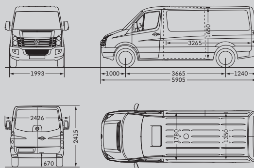
Crafter 30/35 Delivery Van with medium wheelbase and normal roof
