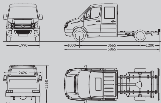
Crafter 35 Chassis with double cab and medium wheelbase
