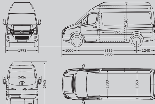
Crafter 35 Delivery Van with medium wheelbase and super-high roof
