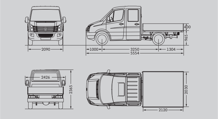
Crafter 30 Dropside Van with double cab and short wheelbase
