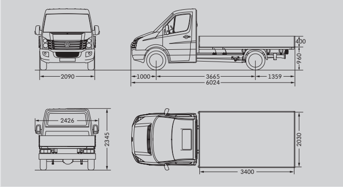
Crafter 35 Dropside Van with single cab and medium wheelbase
