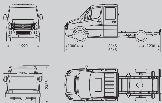
Crafter 30 Chassis with double cab and medium wheelbase
