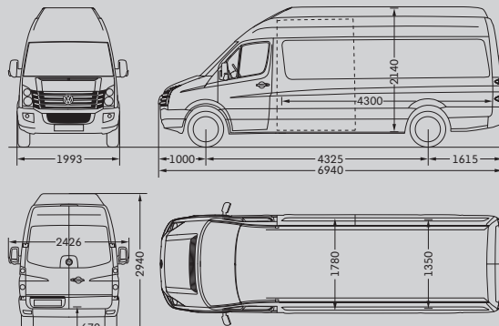
Crafter 35 Delivery Van with long wheelbase and super-high roof
