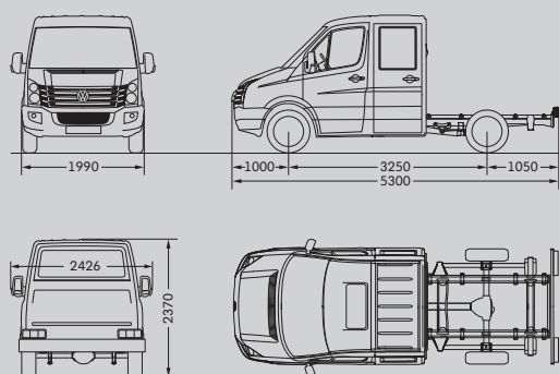
Crafter 35 Chassis with double cab and short wheelbase
