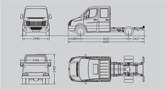
Crafter 50 Chassis with double cab and medium wheelbase
