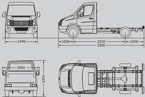
Crafter 35 Chassis with single cab and short wheelbase
