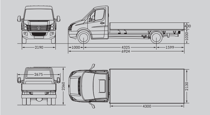
Crafter 50 Dropside Van with single cab and long wheelbase
