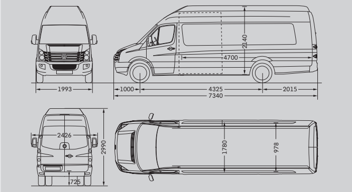
Crafter 50 Delivery Van with long wheelbase, overhang and super-high roof
