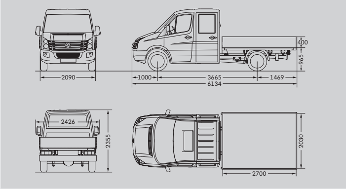
Crafter 30 Dropside Van with double cab and medium wheelbase
