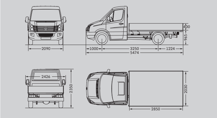
Crafter 30 Dropside Van with single cab and short wheelbase
