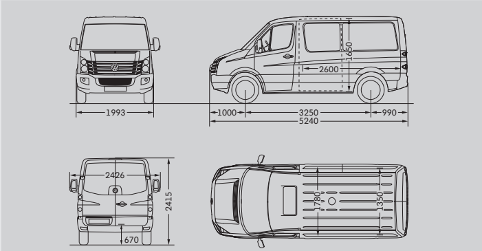
Crafter 30/35 Kombi with short wheelbase and normal roof
